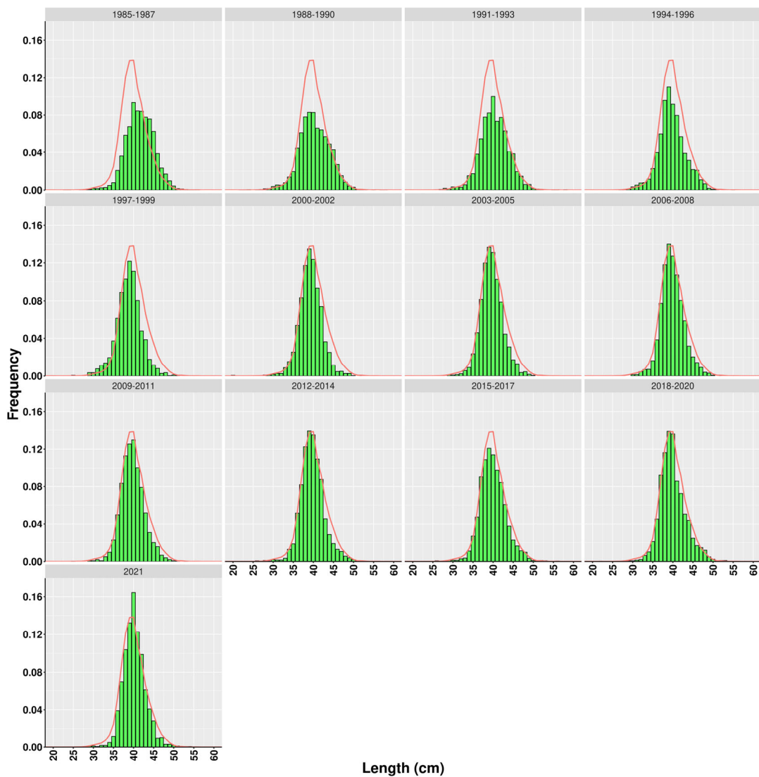
Fig. 11. Lumpfish. Length distribution of female lumpfish caught in the IS-SMB grouped into three year periods for 1985-2021. Lines represent the average length distribution for the whole study period.
