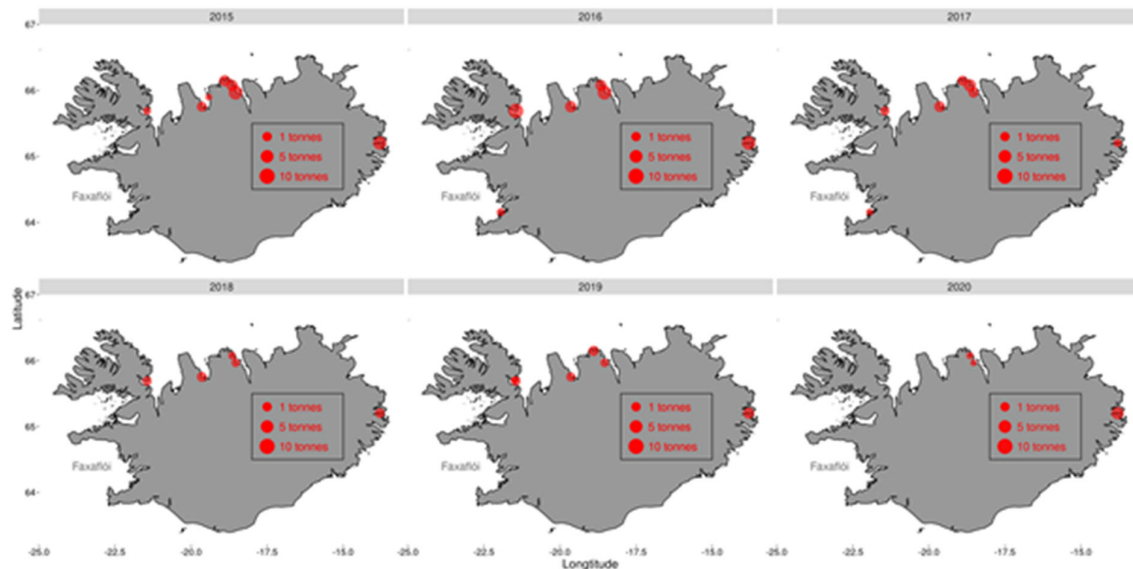
Fig. 4. Lumpfish. Landings of male lumpfish from the directed male fishery by harbour 2015-2020.
