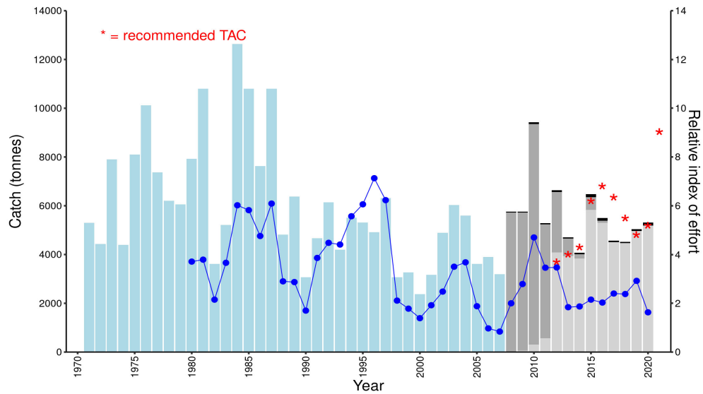
Fig. 3. Lumpfish. Landings of females between 1970 and 2021 (bars) and lumpfish gillnet effort index for the female fishery 1980-2020 (blue line). Blue bars represents landings estimated from barrels of roe. Dark grey represents landings of roe converted to weight of whole lumpfish, and light grey represents landings of whole lumpfish. Black represents landings from other fisheries. The recommended TAC for each year is shown with red asterisks.
