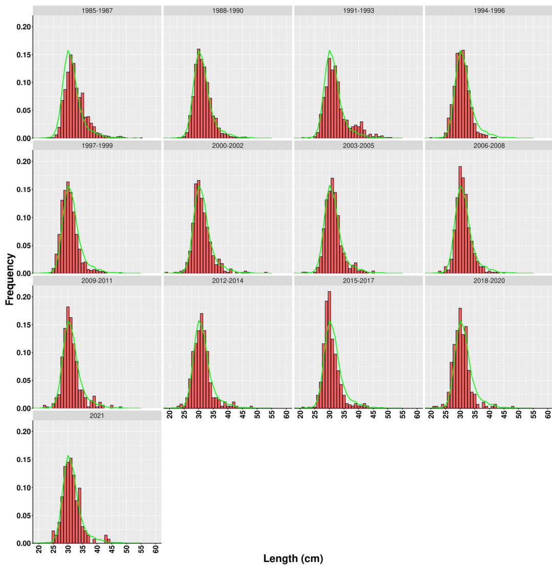
Fig. 13. Lumpfish. Length distribution of male lumpfish caught in the IS-SMB grouped into three year periods for 1985-2021. Lines represent the average length distribution for the whole study period.
