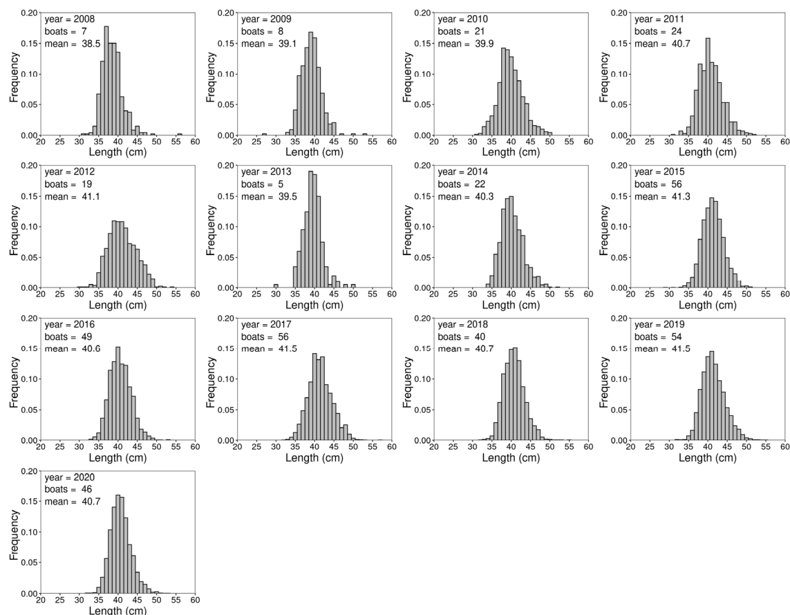
Fig. 7. Lumpfish. Length distribution of females from the female fishery from 2008-2020. The number of boats sampled and mean length is given. Forty fish are measured from each boat sample.
