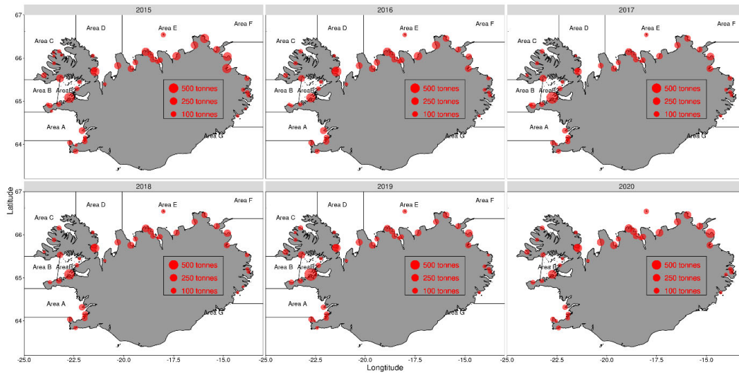
Fig. 2. Lumpfish. Landings of female lumpfish by harbour 2015-2020. Lumpfish management areas are shown. In 2020, there were only two management areas.
