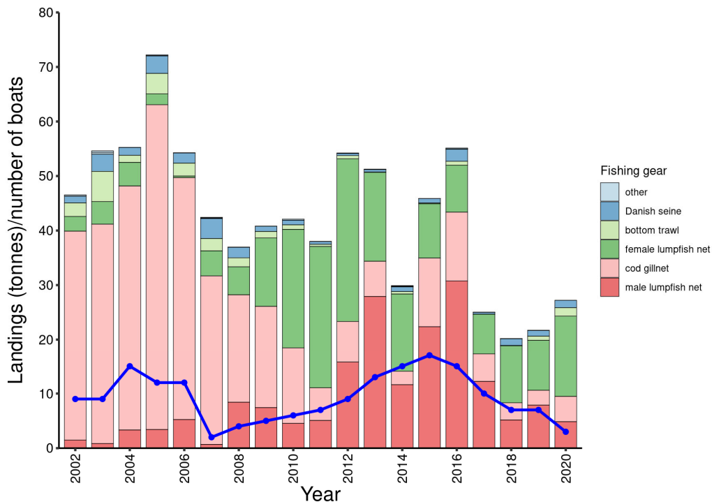
Fig. 5. Lumpfish. Landings of male lumpfish between 2002 and 2020 by gear type. Blue line shows the number of boats which participated in the male fishery.
