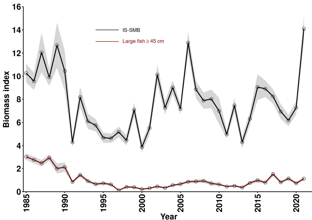
Fig. 9. Lumpfish. Biomass index of female lumpfish and biomass index of large lumpfish \geq 45 cm in March from the IS-SMB from 1985-2021.
