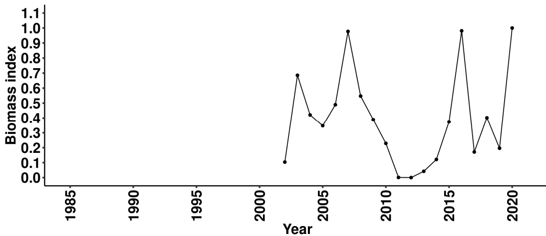
Fig. 10. Lumpfish. Biomass index of lumpfish from the gillnet survey (SMN) from 2002-2020. Note that it is not separated by sex.
