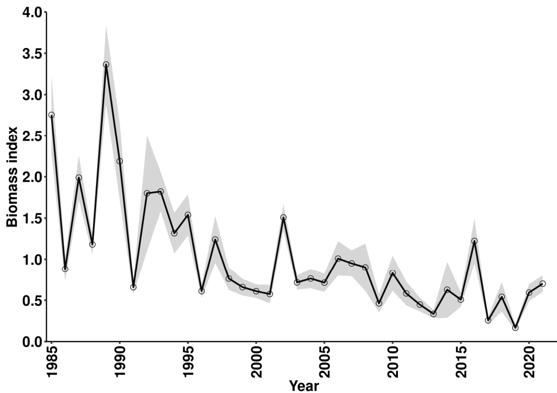
Fig. 12. Lumpfish. Biomass index of males from the IS-SMB for 1985-2021.
