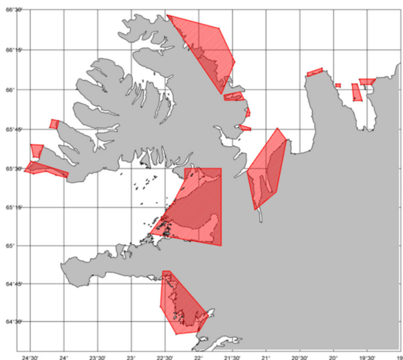
Fig. 6. Lumpfish. Areas closed to lumpfish fishing to reduce the risk of marine mammal bycatch.
