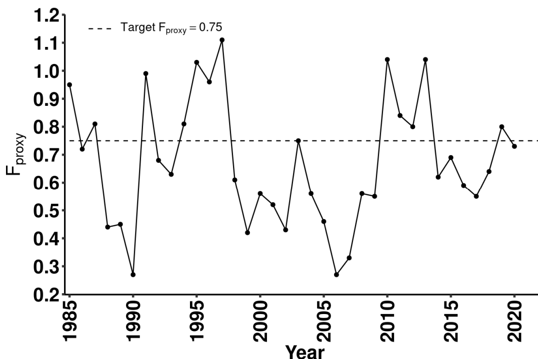
Fig. 14. Lumpfish. F_{\text{proxy}} of females 1985–2020. Target F_{\text{proxy}} is shown (dashed line).
