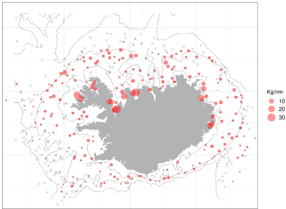
Figure 12. Long rough dab. Spatial distribution of long rough dab in the autumn survey in 2021.
