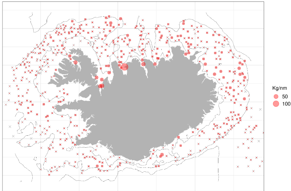
Figure 10. Long rough dab. Spatial distribution in the spring survey in 2022.
